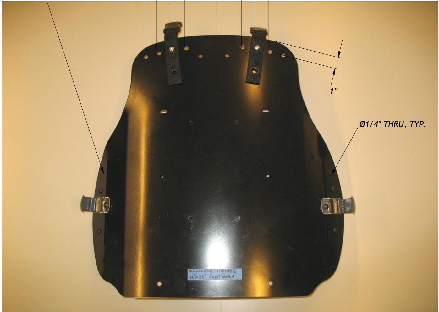
LOWER STRAPS CAN BE FITTED TO EXISTING SLOTS USING WELD NUTS
